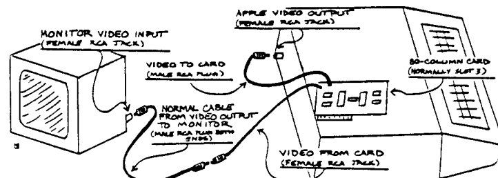
FIGURE 1: TYPICAL 80-COLUMN CARD HOOKUP (APPLE ][ AND APPLE ][+)
